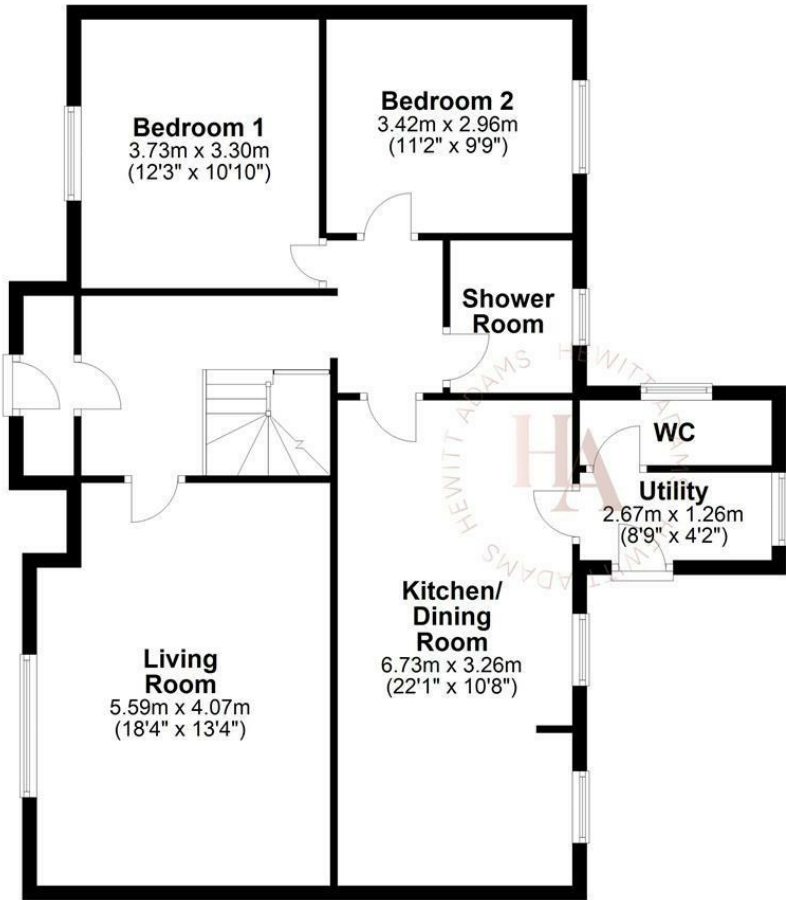
Ground Floor Approx. 92.8 sq. metres (999.4 sq. feet)
